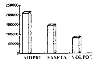
Fig. 3.3 Memory requirements in bytes
