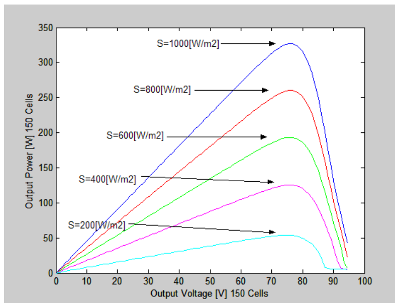
Fig. 7 Irradiation Power Curve for T= 25^\circ\text{C}
