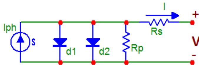
Figure 4: Equivalent Circuit of a Solar Cell
