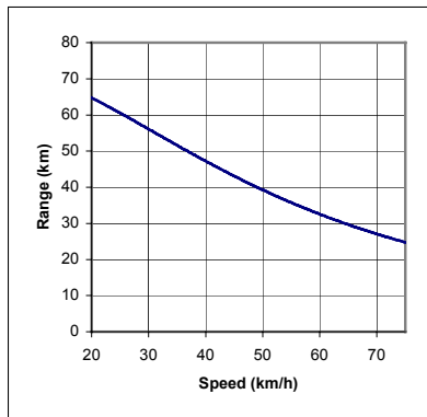
Fig. 11 Range as a function of speed in a small EV
