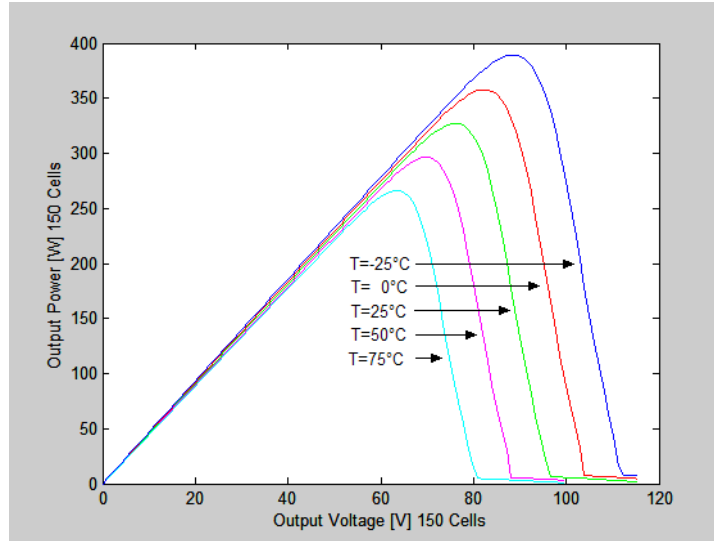
Fig. 8 Temperature Power Curve for S=1000 \text{ [W/m}^2\text{]}
