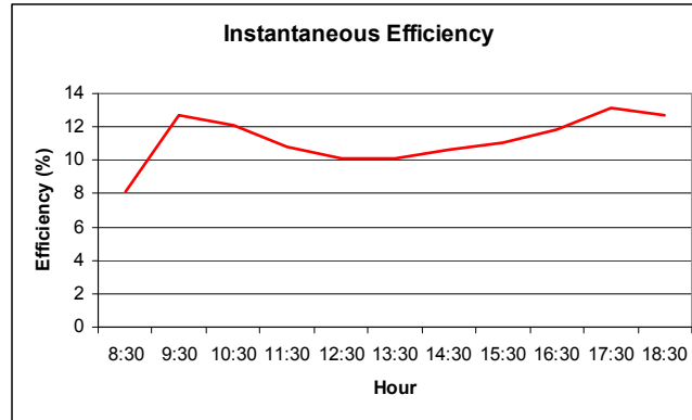
Fig. 9 Instantaneous Cells Efficiency
