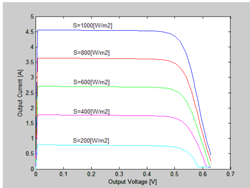
Figure 5: Irradiation Curves for T= 25°C
