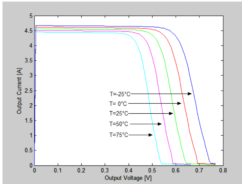
Figure 6: Temperature Curves for S=1000 \text{ [W/m}^2\text{]}
