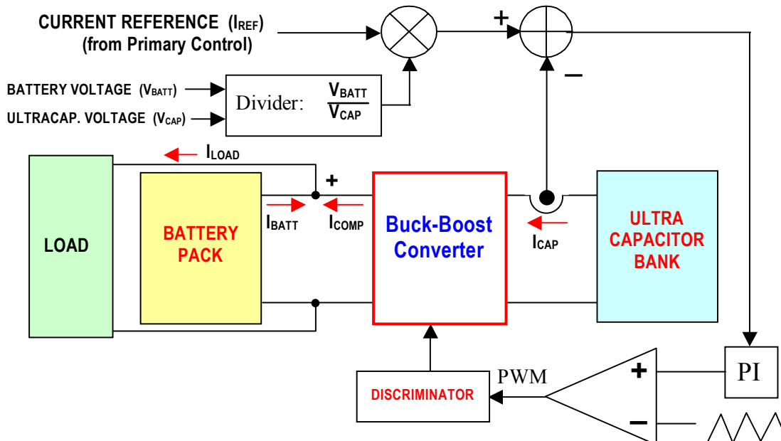
Figure 3 Secondary Control
