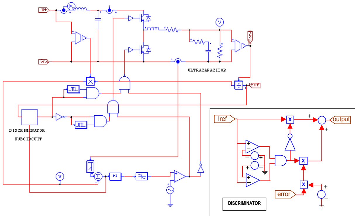
Figure 8 Ultracapacitor Subcircuit
