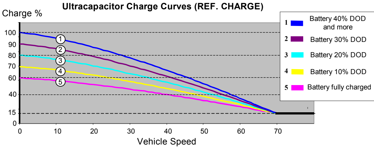
Figure 4 Family plots of the Reference Table, to evaluate the reference charge.
