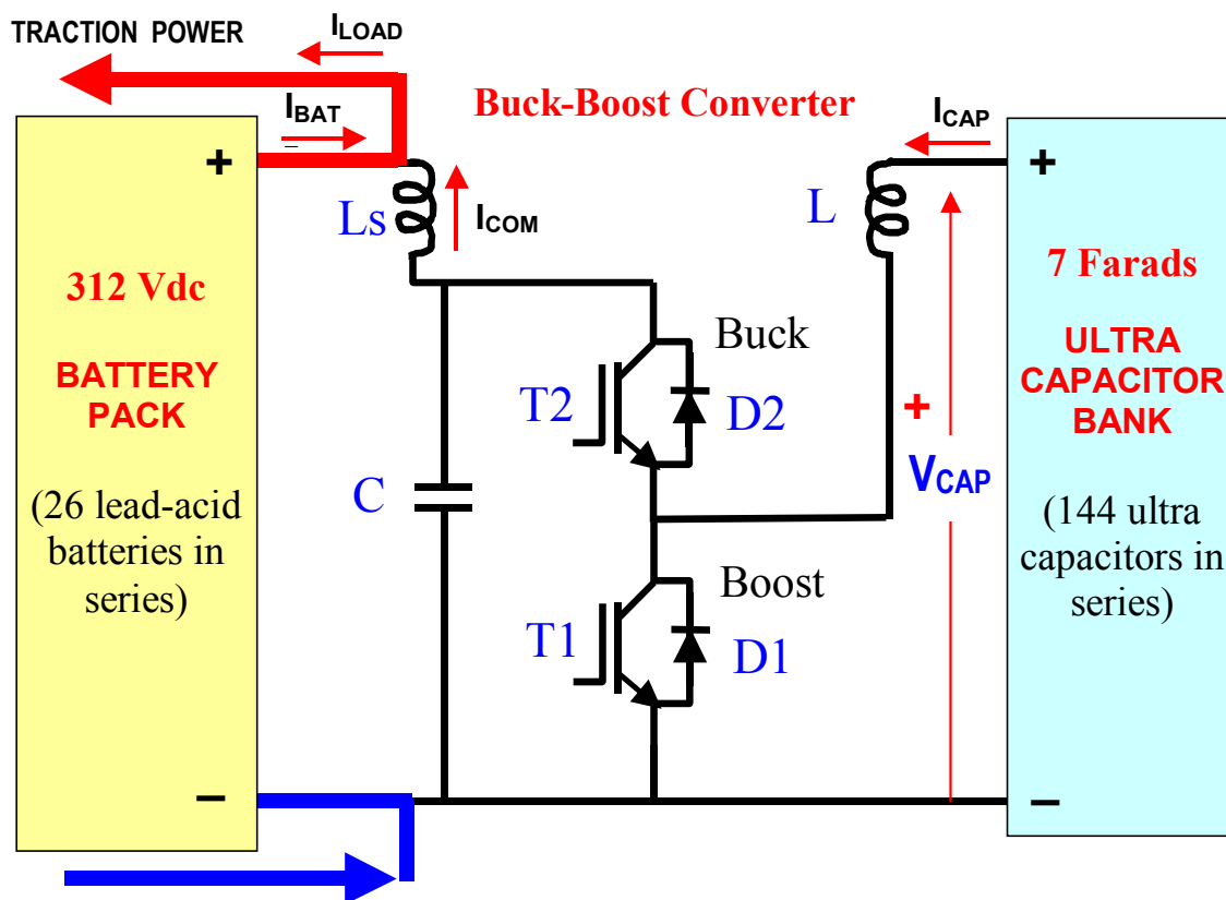
Figure 1 Ultracapacitor System
