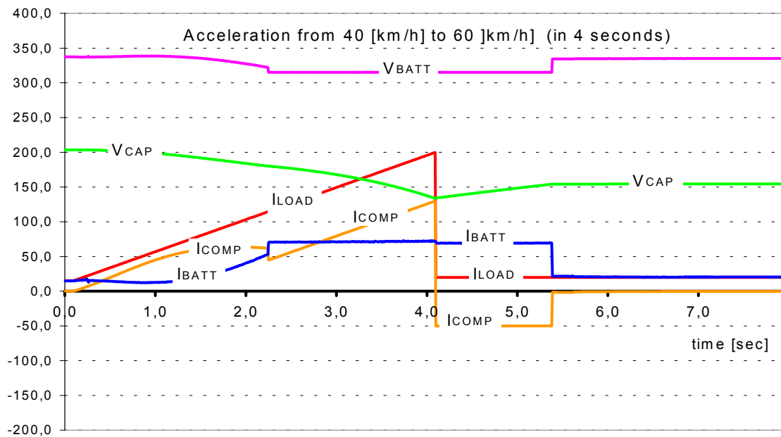
Figure 9 Acceleration from 40 to 60 [km/h]
