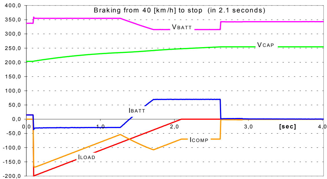
Figure 10 Braking from 40 [km/h] to zero
