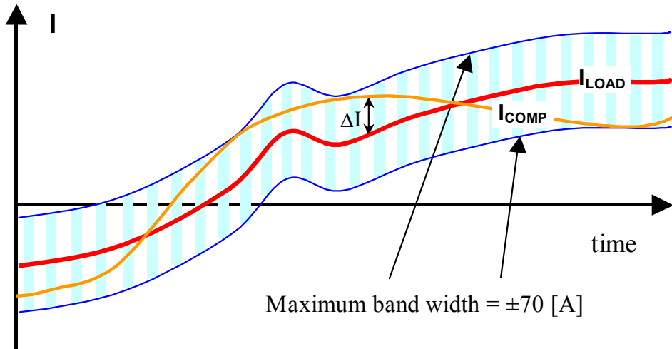
Figure 5 Limiter Block action.
