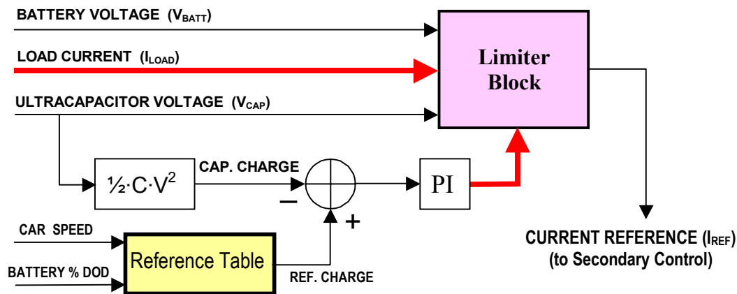
Figure 2 Primary Control
