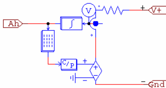
Figure 7 Battery Subcircuit
